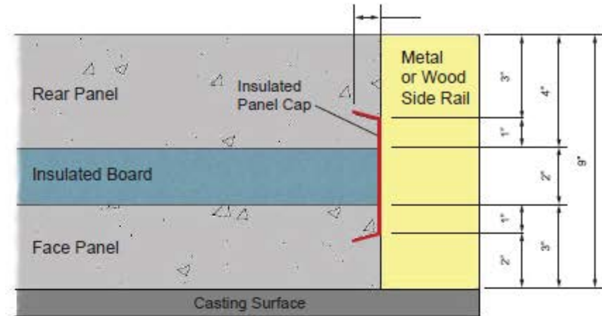
Installation detail for 9" panel
