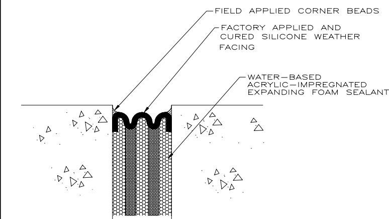
FIGURE 1: COLORSEAL in Typical Installation (substrates may vary).
